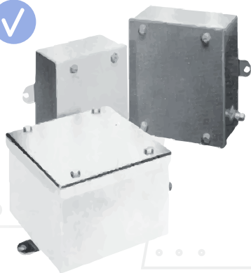
Terminal Boxes Metal (SS316L, Alu) Ex-Cell series -60C to +135C N-TB series -55C to +120C S-TB series -55 to +120C Abox series -55 to +120C Ex e, Ex ia
